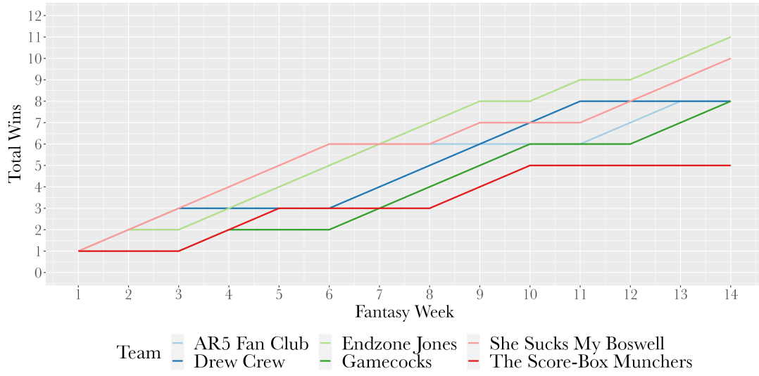
Figure 10: Peach Division Total Wins per Week
