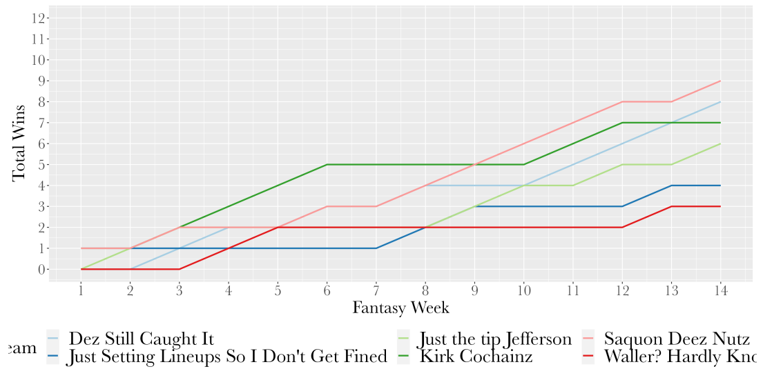
Figure 9: Waluigi Division Total Wins per Week
