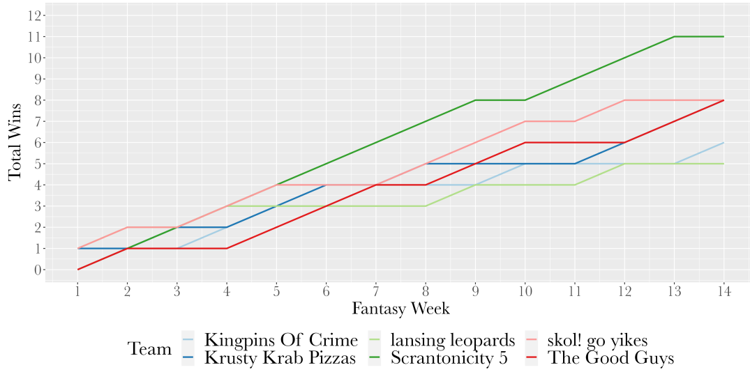
Figure 8: Wario Division Total Wins per Week
