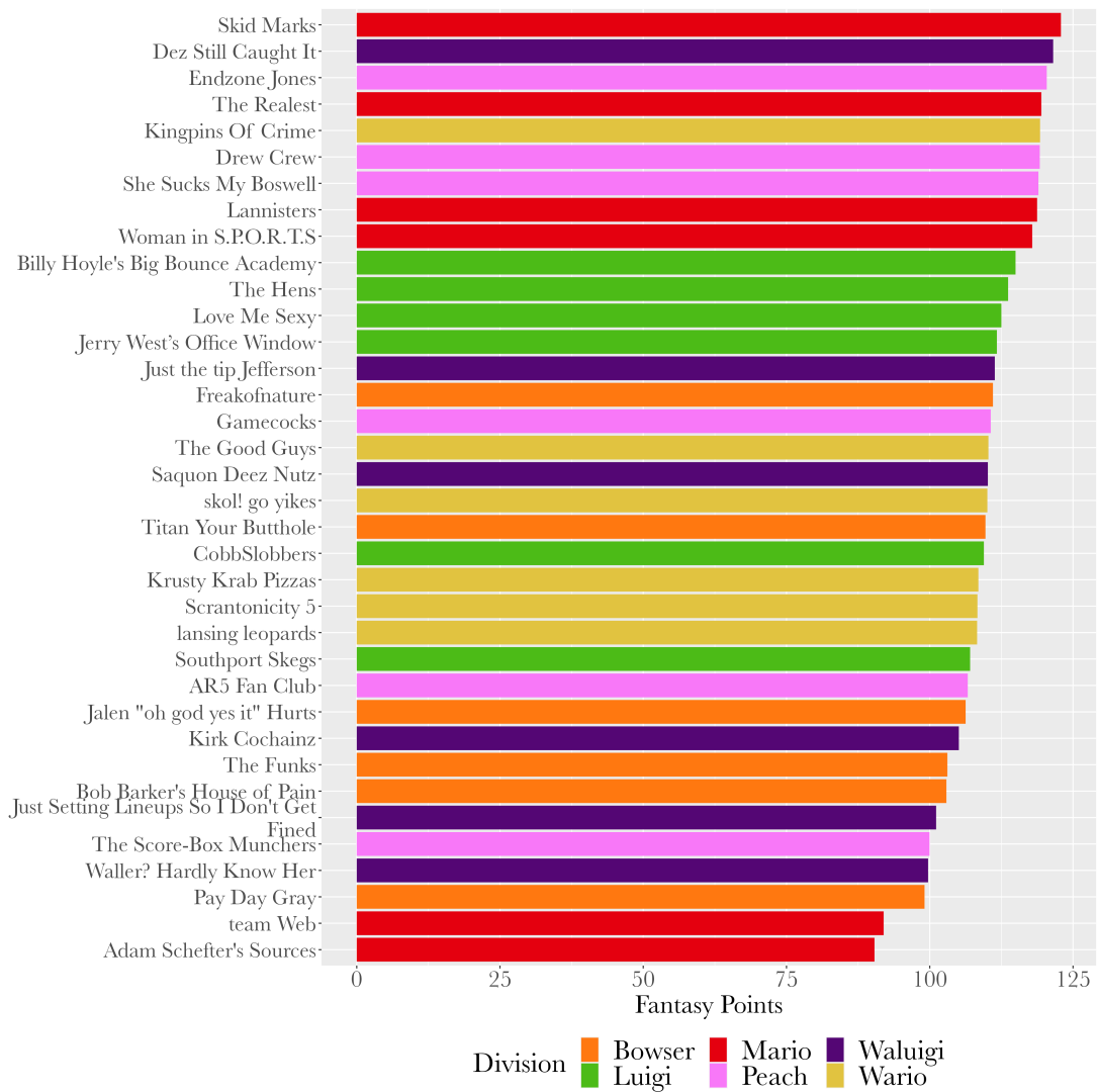
Figure 3: Average Weekly Points by Team
