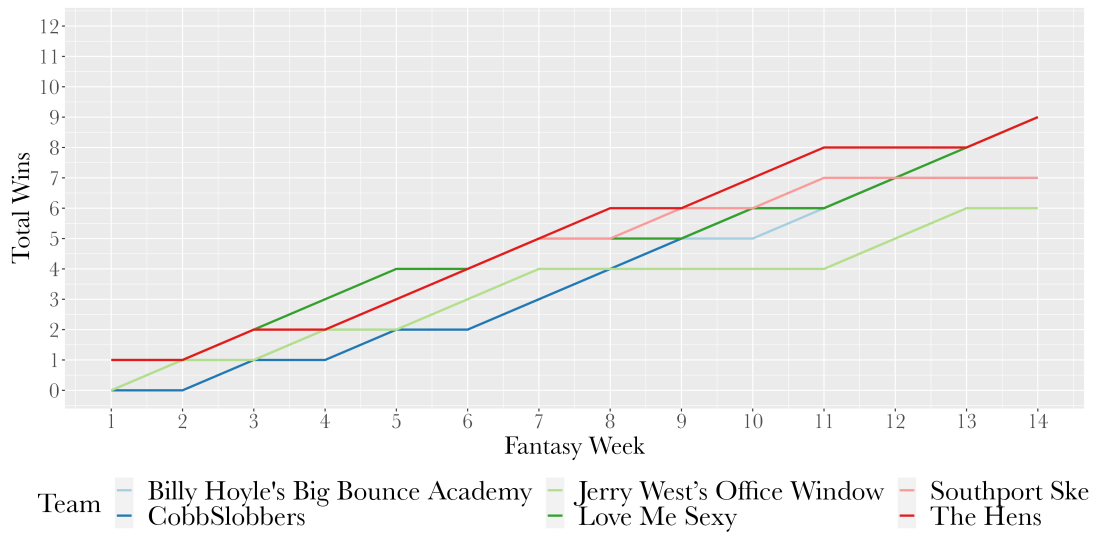
Figure 7: Luigi Division Total Wins per Week
