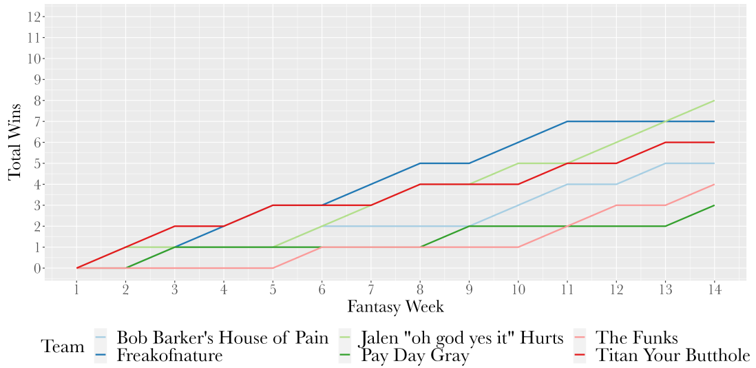
Figure 6: Bowser Division Total Wins per Week
