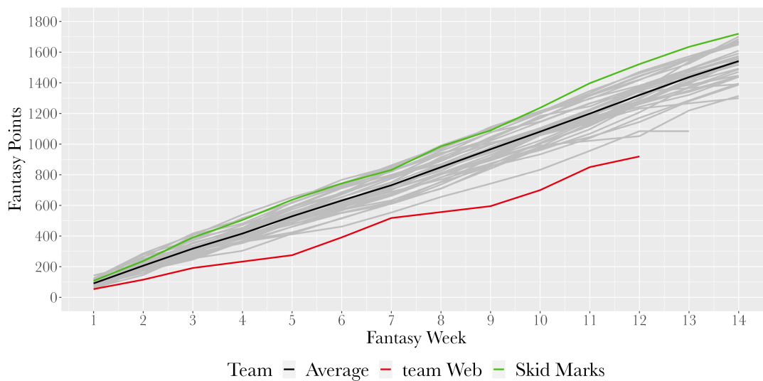
Figure 2: Average Weekly Points Per Roster
