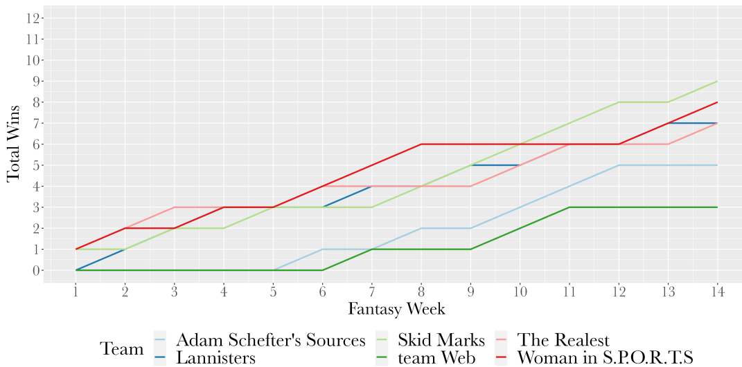
Figure 5: Mario Division Total Wins per Week
