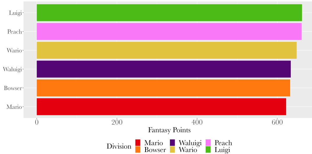
Figure 4: Average Weekly Points by Division
